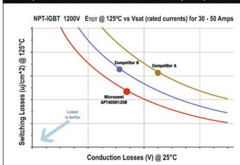
Comparison of new Microsemi 1200V NPT IGBT with major competitors
